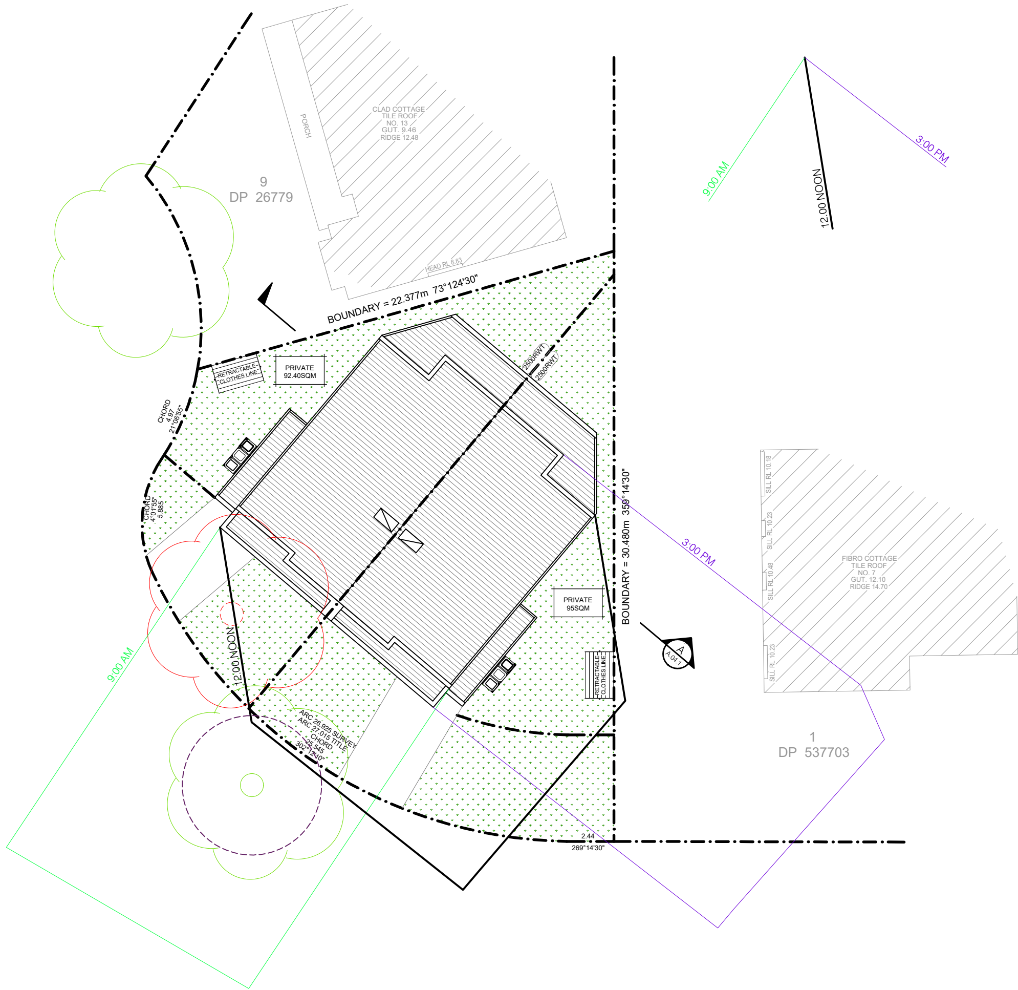
PROPOSED SHADOW DIAGRAM 9AM, 12PM & 3PM SCALE - 1 : 200
